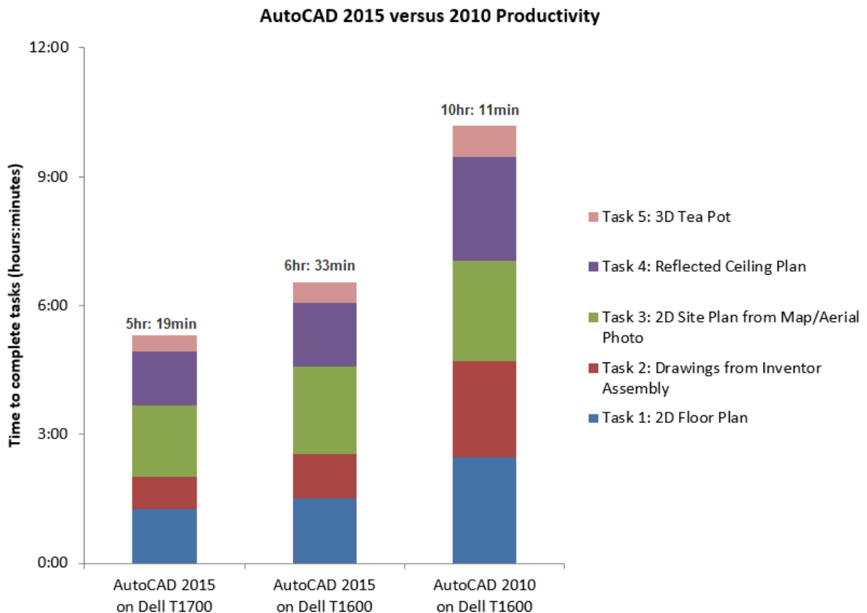
Time to complete all five drawing tasks in AutoCAD 2015 versus AutoCAD 2010.
